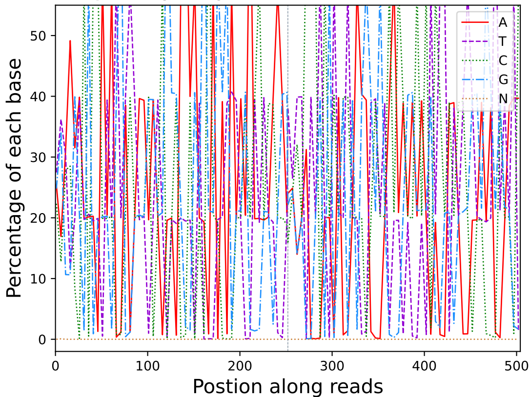
Base percentage along reads (R10104)
